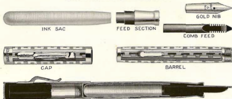
SECTIONAL VIEW
